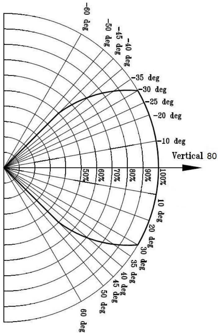
Figure 2-2: Vertical field of view for SharpEye 40/40C-I, C-LB, C-L4B, D-I, D-LB, and D-L4B
